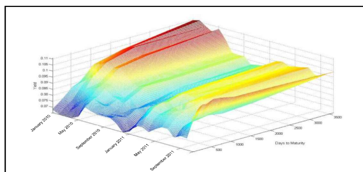
Graph 1: Evolution of TRY Yield Curves
