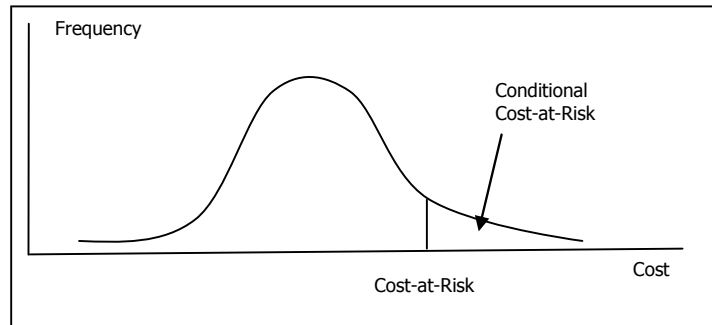
Figure 1: Conditional Cost-at-Risk Approach
