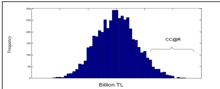
Graph 2: Distribution of Interest Costs
