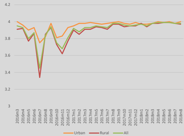
Average hours of electricity supply between 6-10PM
