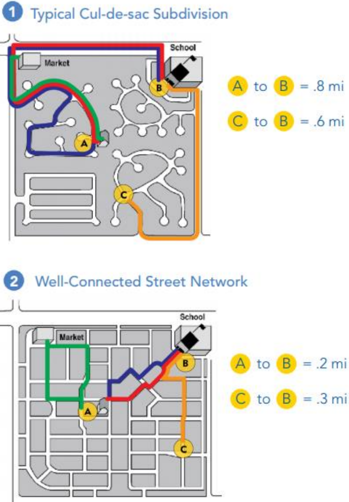
Figure 13: Greater street connectivity reduces trip lengths
